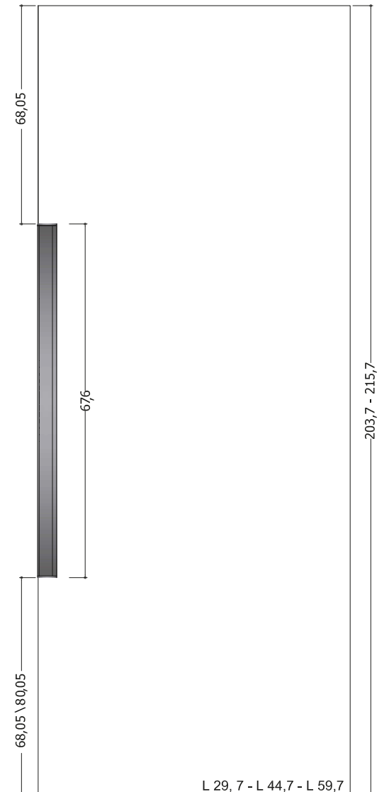
Anta monoporta con maniglia in verticale Single-door with vertical handle
