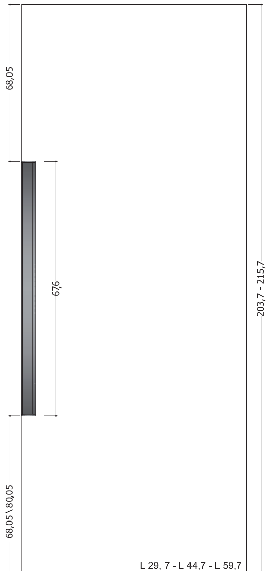
Anta monoporta con maniglia in verticale Single-door with vertical handle
